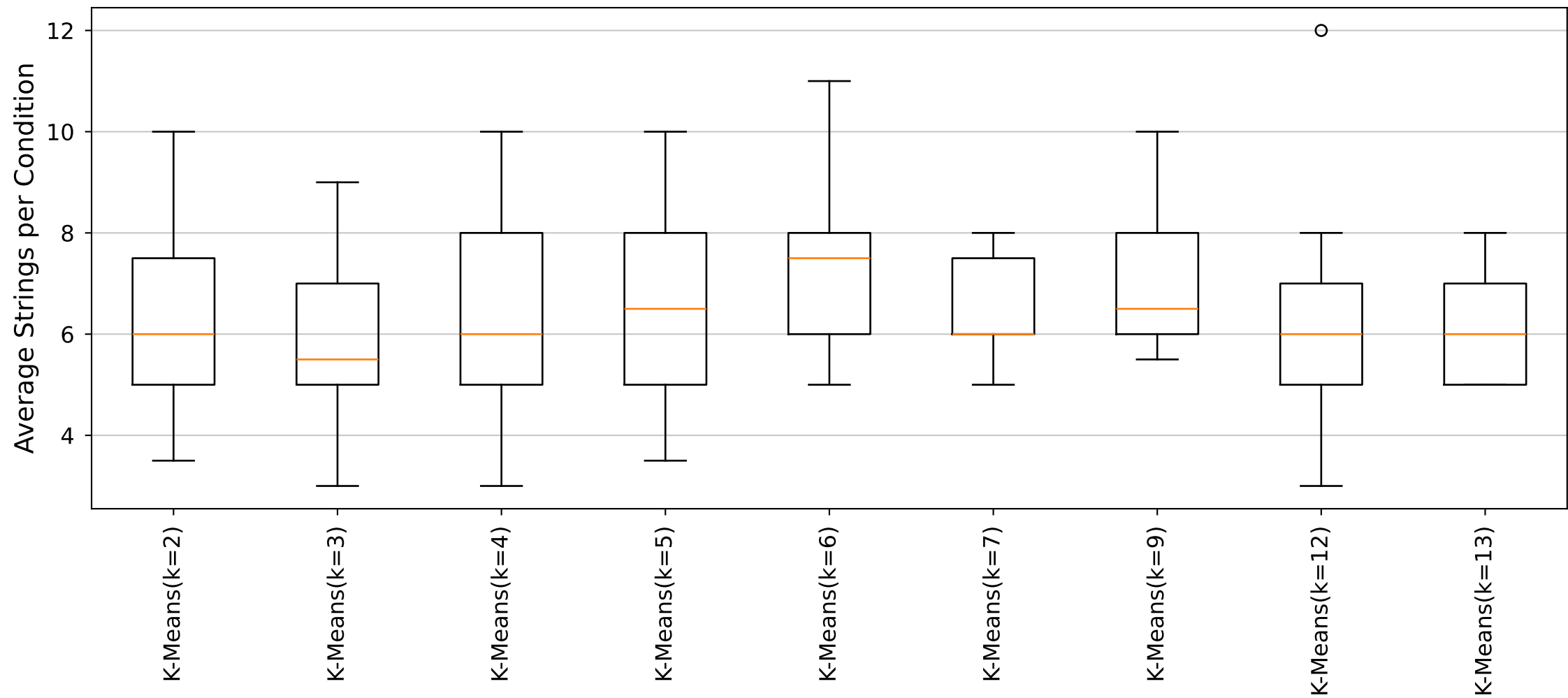
YARA Rules Average Strings per Condition Distribution (Cluster8_Size13 dataset)
